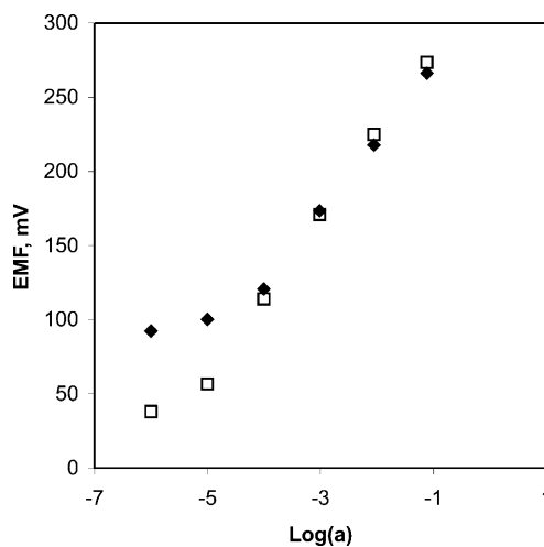
Fig. 9. Typical potentiometric response of \text{K}^+ ion selective electrodes: (◆) PVC; (□) PolyHIPE membrane.
